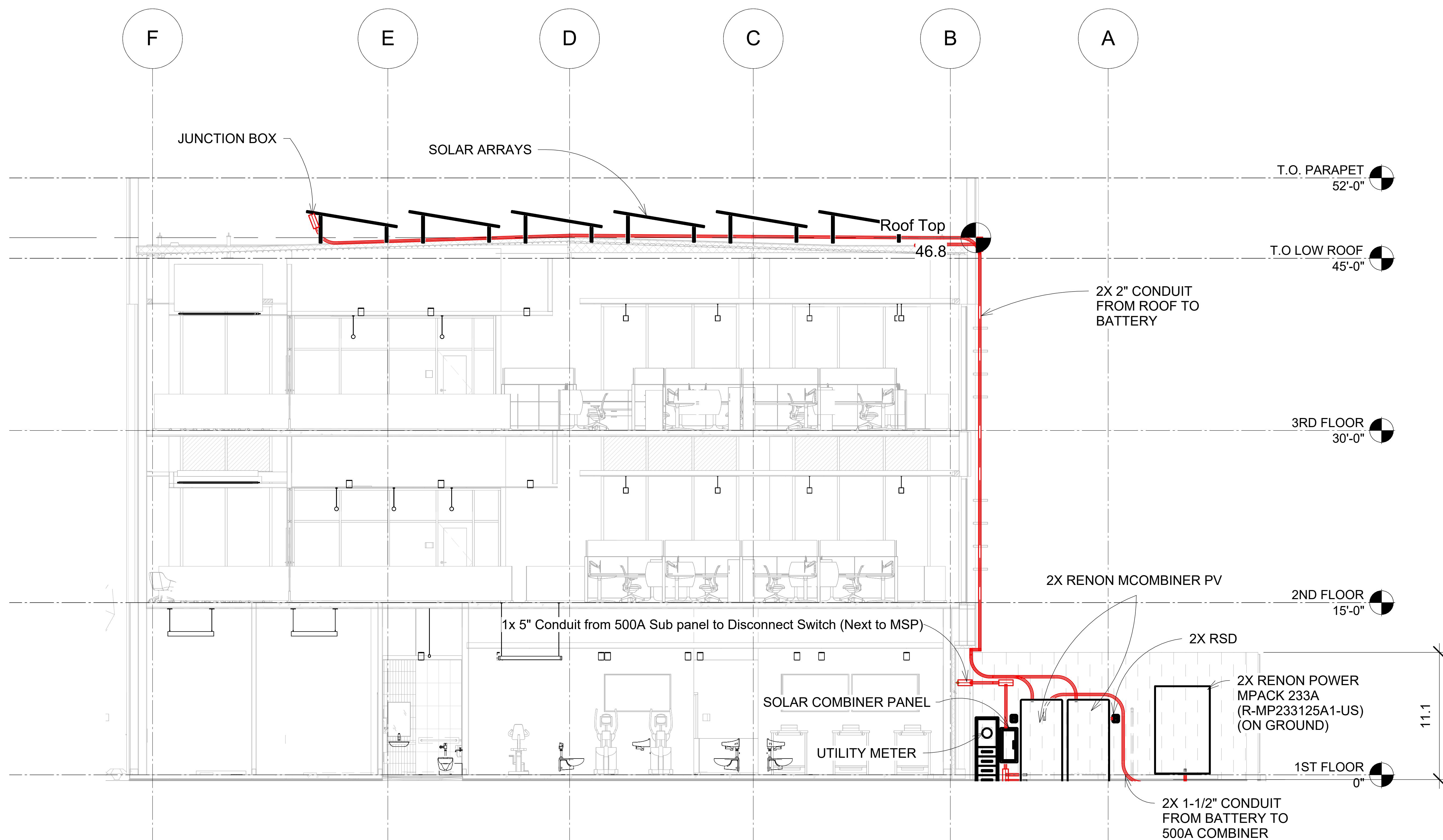
PV EQUIPMENT WEST SIDE CROSS SECTION VIEW
